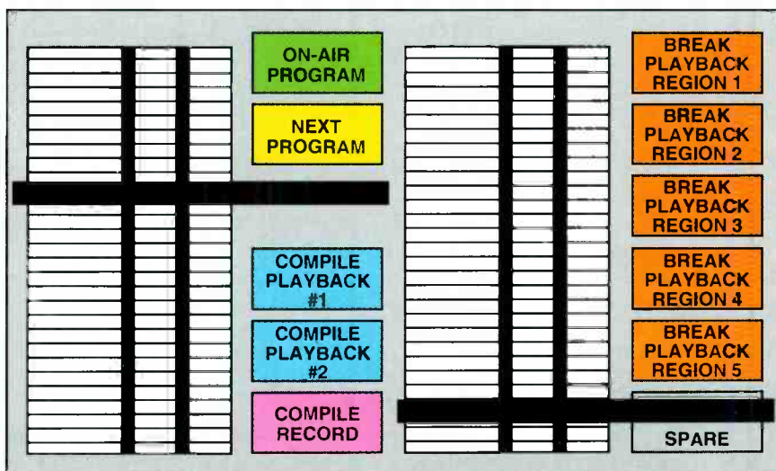
Figure 3. VTR allocation and layout of a cart machine system for multiregional spot insertion.
