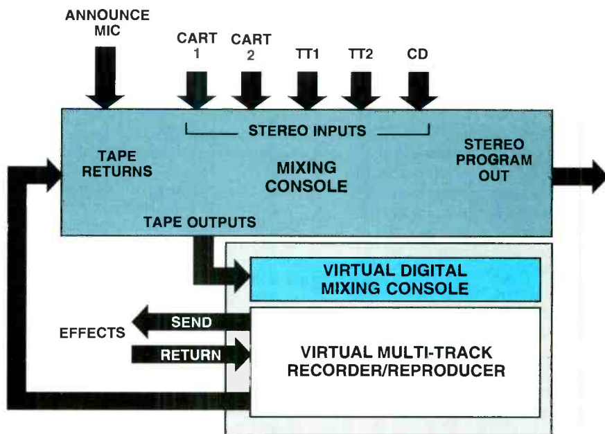
Figure 2. A production studio incorporating a virtual multitrack digital production system. Note that the existing analog mixing console and other traditional hardware may still be included in this hybrid configuration, and that the number of recording tracks may be greater than the number of inputs and outputs on the recorder.
