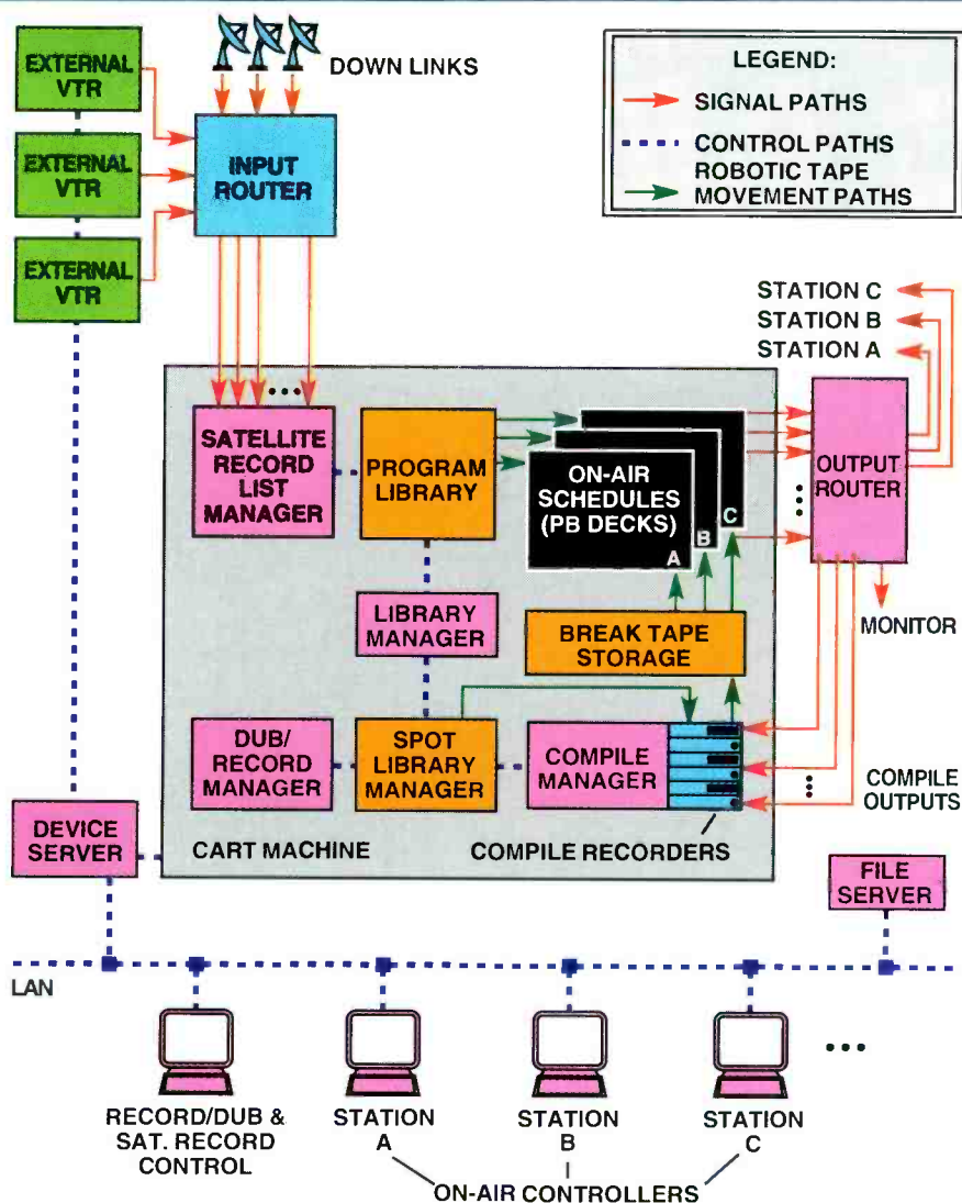
Figure 2. An advanced multicast operation that allows multiple stations to be served with independent, asynchronous schedules from a single storage/playback system.
