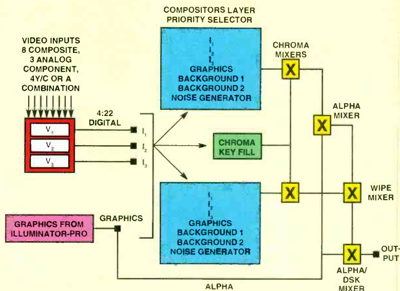
Figure 1. A block diagram of the Matrox SIESTA device.
