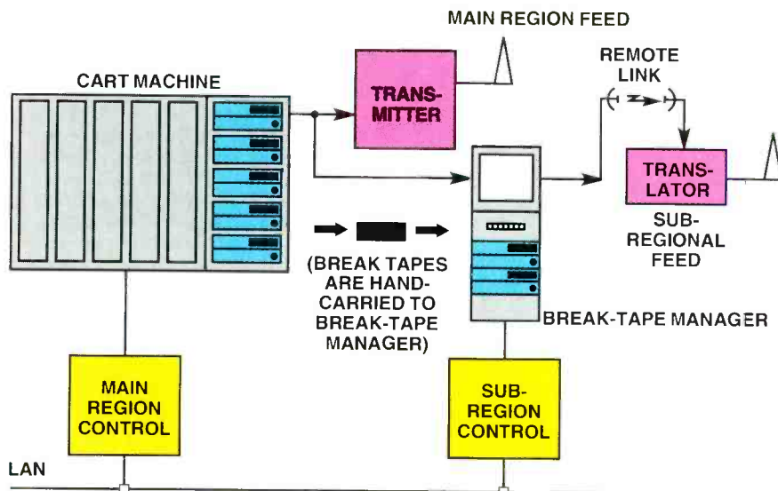
Figure 1. One approach to multicasting, where two stations share the bulk of their programming, with occasional segments split between stations.
