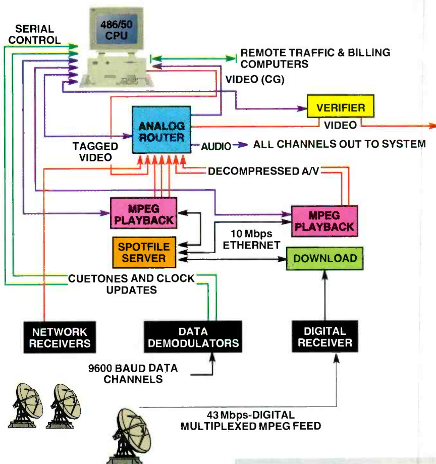
Figure 1. Digital satellite delivery of commercials can tie even the most remote cable systems together as an interconnect, or transport national and promotional spots for near immediate turnaround.
